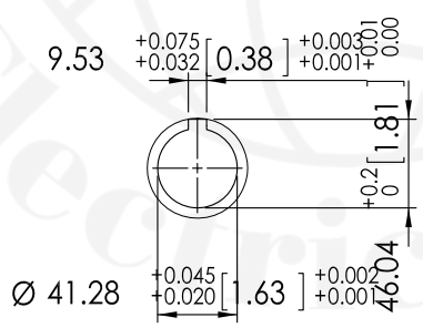
input bore
